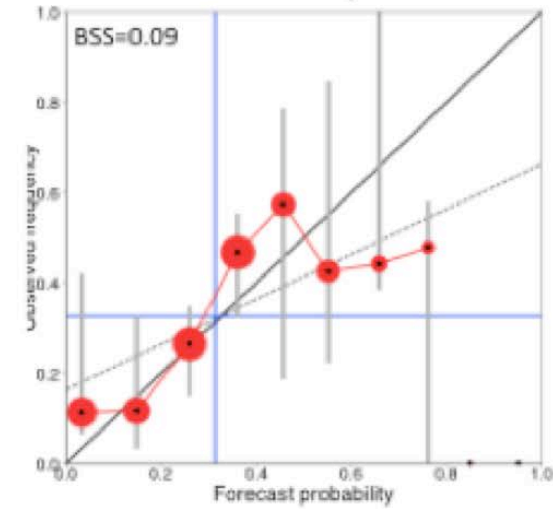
d) NON-INITIALISED Hindcasts SST North Atlantic 2-5yr – lower tercile
