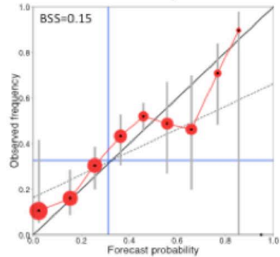
c) INITIALISED Hindcasts SST North Atlantic 2-5yr – lower tercile
