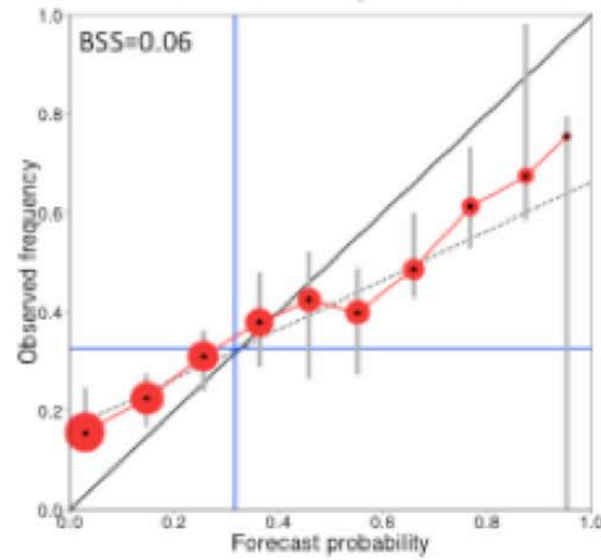
c) INITIALISED Hindcasts SST North Atlantic 2-5yr – lower tercile
