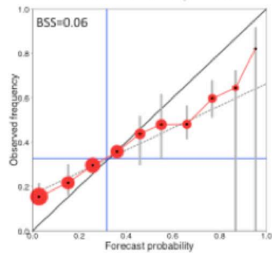
d) NON-INITIALISED Hindcasts SST North Atlantic 2-5yr – lower tercile
