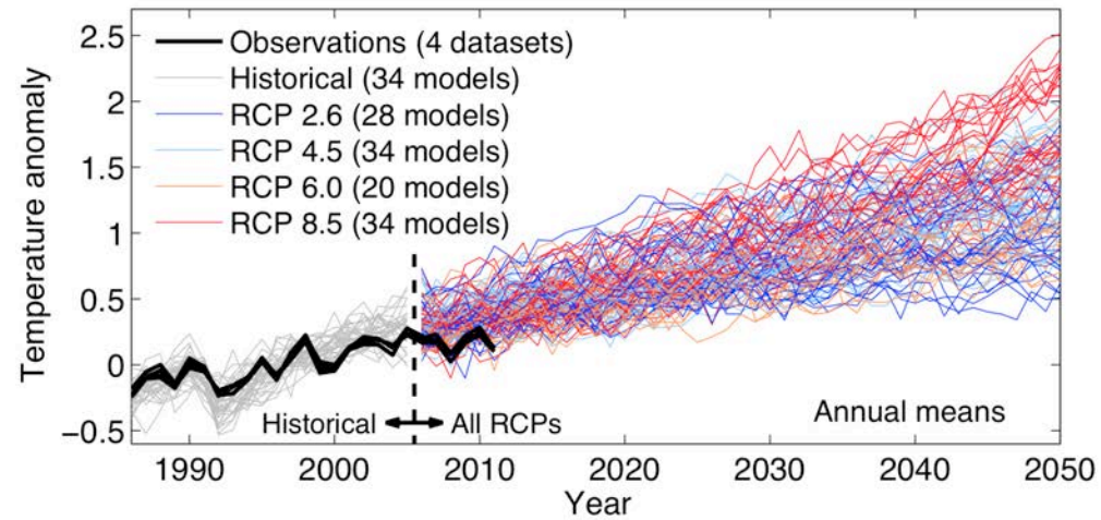
Global mean temperature near-term projections relative to 1986–2005
