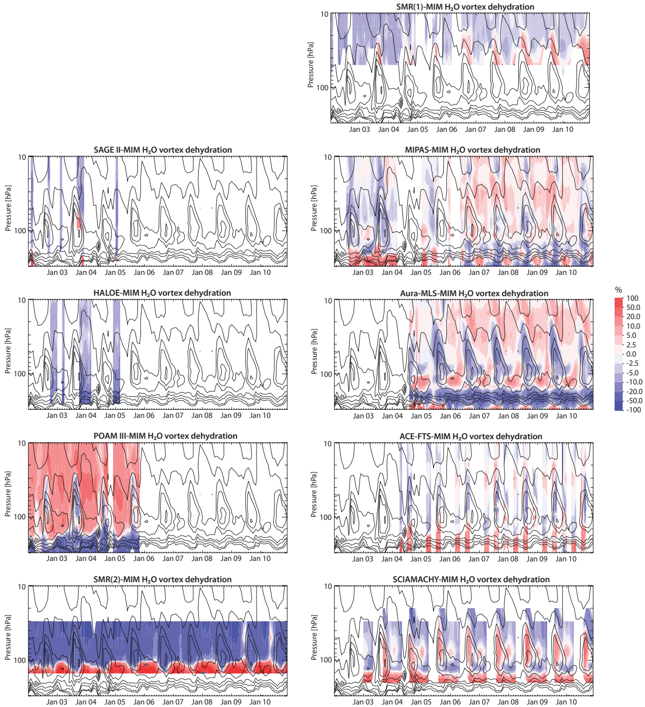
Figure 4.2.21b: Differences for polar vortex dehydration. The time-altitude evolution of \text{H}_2\text{O} differences relative to the MIM between 2002 and 2010 is shown for each individual instrument (same ordering as in Figure 4.2.21a). Contour levels (2.5, 3, 3.5, 4, 5, 6, 8, 10, 50, 100 ppmv, with the 3-ppmv isopleths labelled) reproduce the MIM from Figure 4.2.21a.
