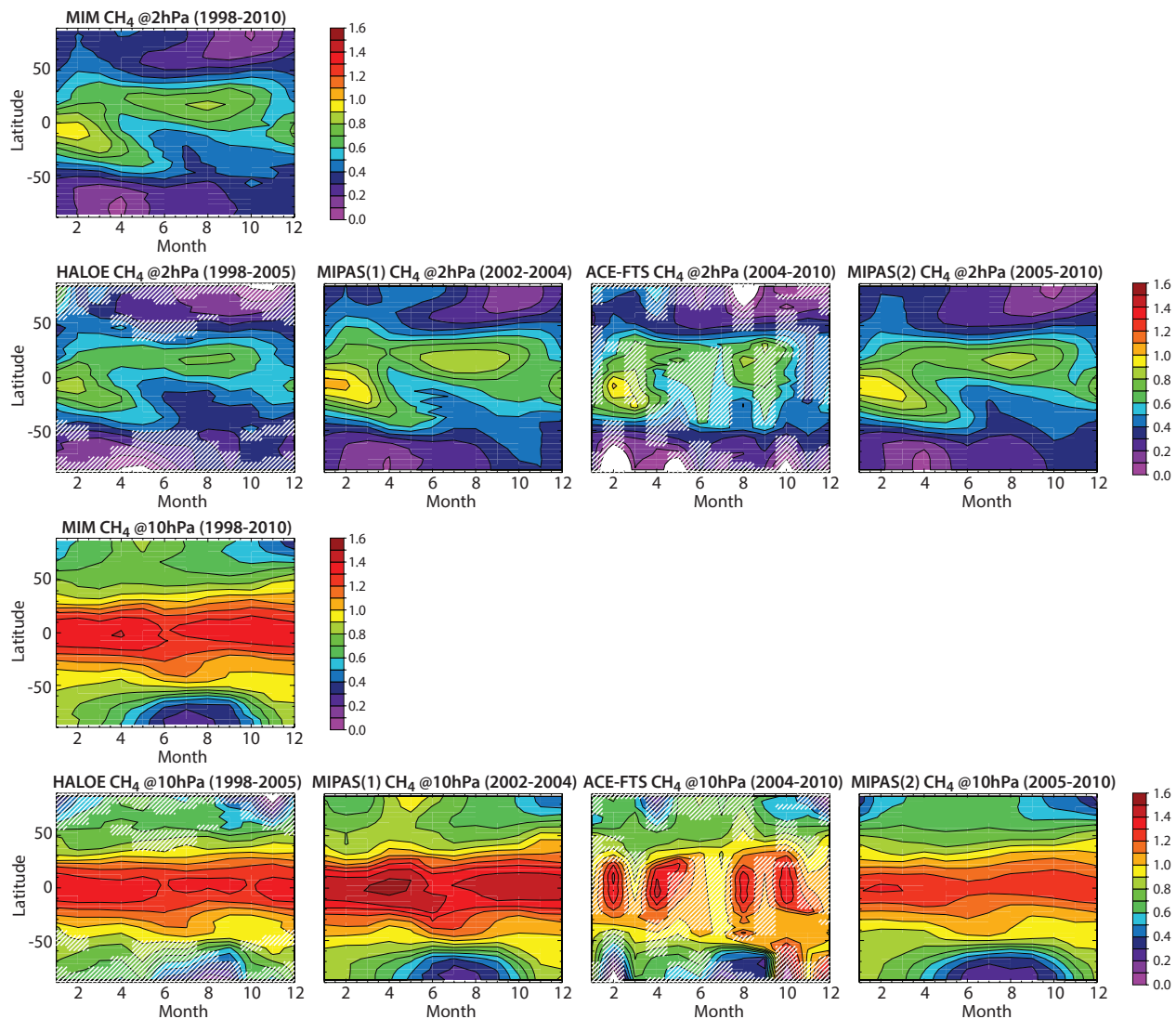
Figure 4.3.4a: Latitude–time evolution of \text{CH}_4 . The latitude–time evolution of monthly zonal mean \text{CH}_4 at 2 hPa (top two rows), and 10 hPa (bottom two rows) are shown for the MIM (1998–2010), HALOE (1998–2005), MIPAS(1) (2002–2004), ACE-FTS (2004–2010), and MIPAS(2) (2005–2010) averaged over the time period given in brackets. HALOE and the ACE-FTS show interpolated fields, with hatched regions indicating where no measurements are available.
