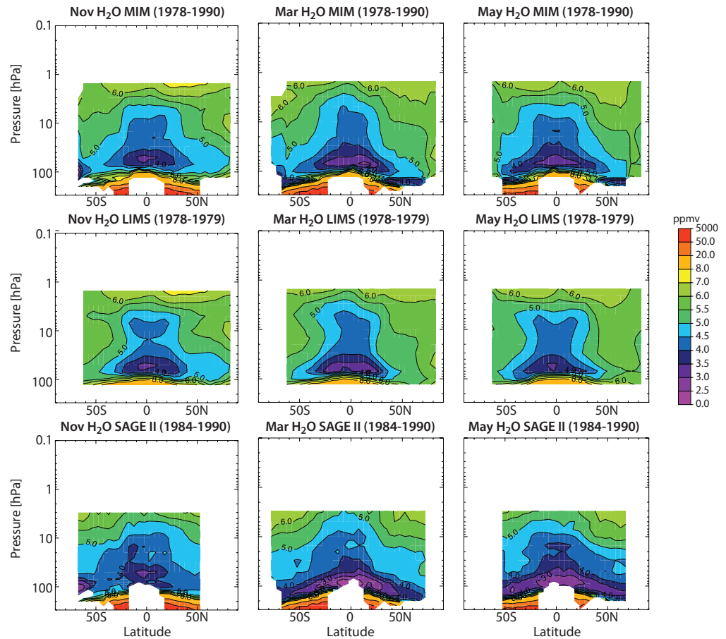
Figure 4.2.1a: Cross sections of monthly zonal mean H_2O for LIMS (1978-1979) and SAGE II (1984-1990). November, March and May monthly zonal means (from left to right) are shown for the MIM, LIMS, and SAGE II (from top to bottom).
