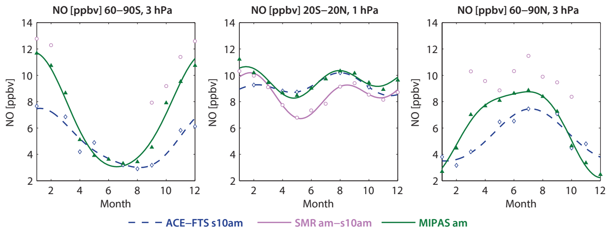
Figure 4.10.9: Seasonal cycle of 10am NO for 2005-2010. Seasonal cycle of monthly zonal mean NO for 60°S-90°S, 3 hPa (left column), 20°S-20°N, 1 hPa (middle column) and 60°N-90°N, 3 hPa (right column). Measurements correspond to 10am LST (MIPAS, filled symbols) or are scaled to 10am LST (ACE-FTS, SMR, open symbols).
