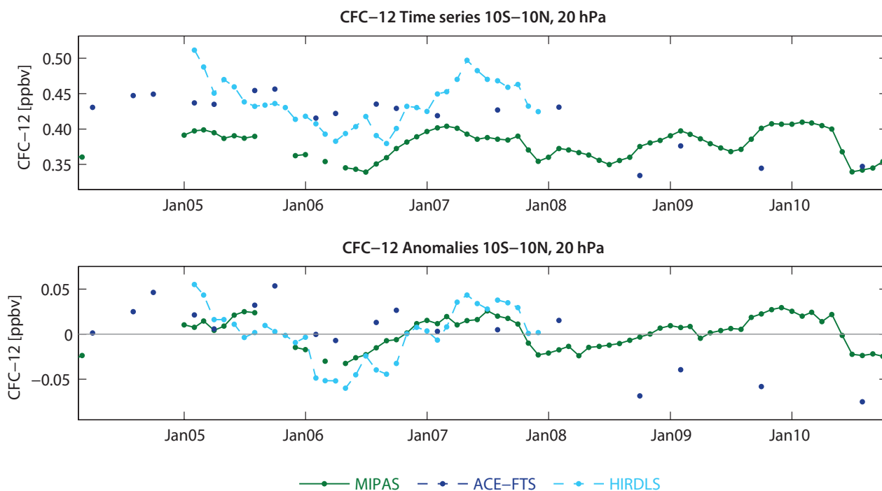
Figure 4.6.5: Time series of CFC-12 monthly mean values and deseasonalised anomalies in the tropics. Monthly mean values (upper panel) and deseasonalised anomalies (lower panel) of CFC-12 between 10°S – 10°N at 20 hPa.
