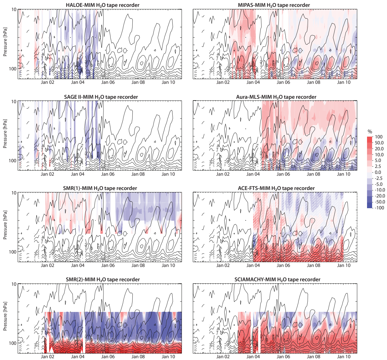
Figure 4.2.16b: Differences for H_2O tape recorder. Altitude-time evolutions of H_2O differences relative to the MIM are shown for the time period 2000-2010 and each individual instrument (same ordering as in Figure 4.2.16a). Contour levels (2.5, 3, 3.5, 4, 5, 6, 8, 10, 50, 100 ppmv, with the 3-ppmv isopleths labelled) reproduce the MIM from Figure 4.2.16a.
