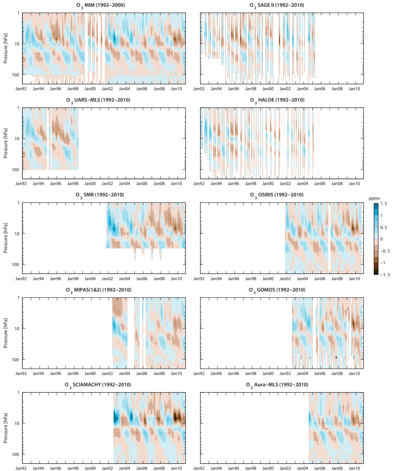
Figure 4.1.25: QBO signal for 1992-2010. Altitude-time sections of deseasonalised ozone anomalies for 10°S-10°N from 1992 to 2010 are shown. The MIM is based on all displayed datasets.
