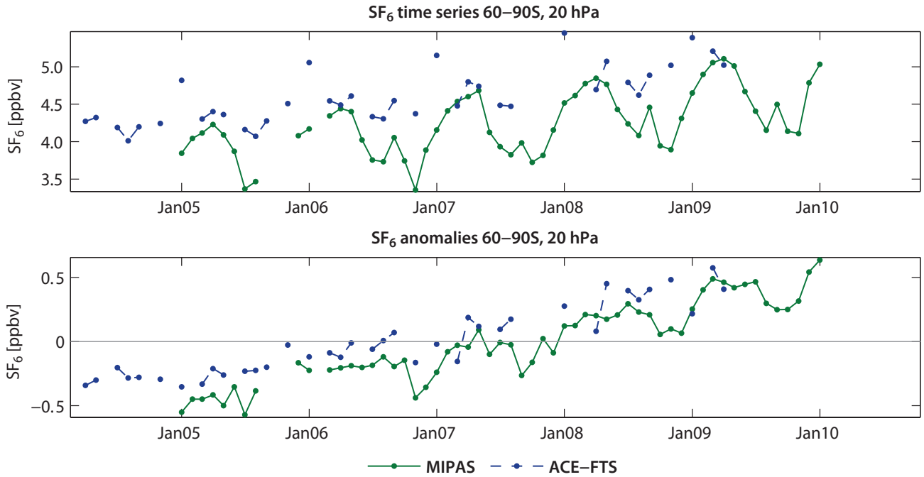
Figure 4.9.6: Time series of \text{SF}_6 monthly mean values and deseasonalised anomalies at SH high latitudes. Monthly mean values (upper panel) and deseasonalised anomalies (lower panel) of \text{SF}_6 between 60^\circ\text{S} - 90^\circ\text{S} at 20 hPa.
