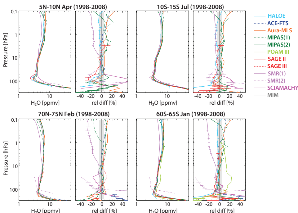
Figure 4.2.13: Vertical profiles of monthly zonal mean H_2O for 1998-2008. The H_2O profiles and their relative differences to the MIM are shown for April 5°N-10°N, July 10°S-15°S, February 70°N-75°N, and January 60°S-65°S. Error bars indicate the uncertainties in the relative differences based on the SEM of each instrument. The grey shaded area indicates where relative differences are smaller than \pm 5\% .
