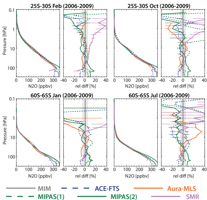
Figure 4.4.2: Vertical profiles of monthly zonal mean N_2O for the Southern Hemisphere. Vertical N_2O profiles for 25°S-30°S February and October (upper panels), and for 60°S-65°S January and July (lower panels) are shown together with the instrument differences from the MIM for SMR, MIPAS(1), ACE-FTS, Aura-MLS, and MIPAS(2) and for the period 2006-2009.
