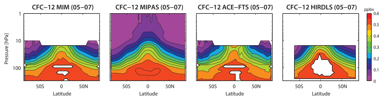
Figure 4.6.1: Cross sections of annual zonal mean CFC-12 for 2005-2007. Annual zonal mean CFC-12 cross sections are shown for the MIM, MIPAS, ACE-FTS, and HIRDLS. The MIM is only displayed for regions where at least two instruments provide measurements.
