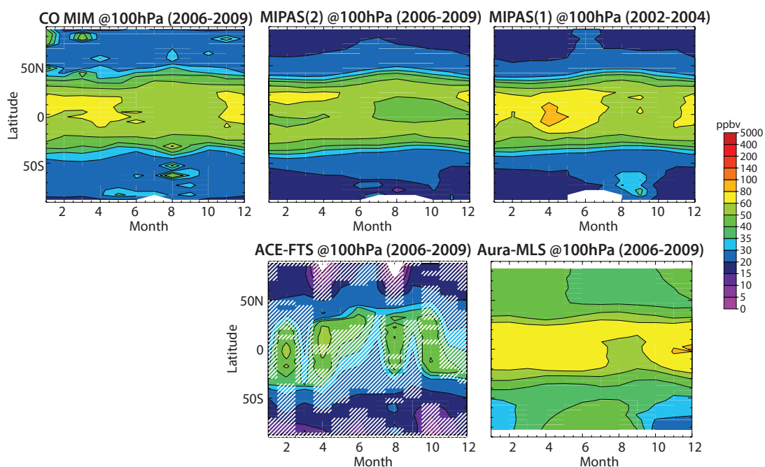
Figure 4.7.4b: Same as Figure 4.7.4a, but for 100 hPa.
