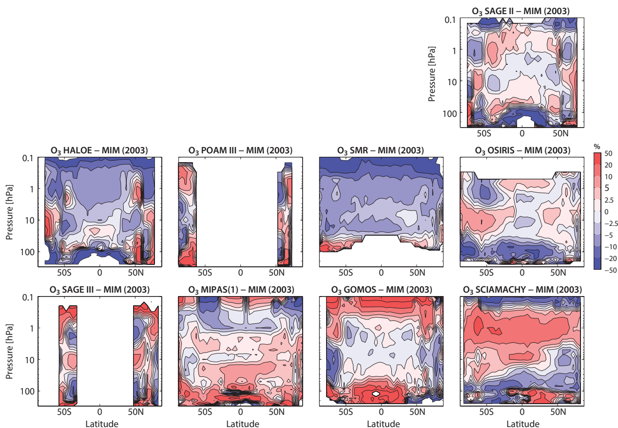
Figure 4.1.7: Cross sections of annual zonal mean ozone differences for 2003. Annual zonal mean ozone differences for 2003 between the individual datasets and the MIM are shown.
