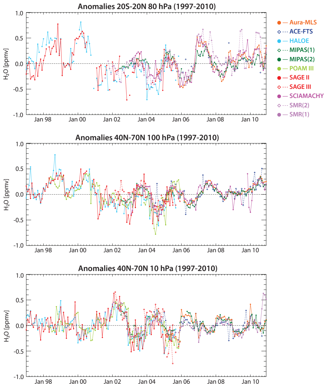
Figure 4.2.22: Time series of deseasonalised anomalies of H_2O for 1997-2010. Time series of deseasonalised anomalies in H_2O at 80 hPa between 20^\circ S and 20^\circ N (upper panel), and at 100 hPa (middle panel) and 10 hPa (lower panel) between 40^\circ N and 70^\circ N , respectively.
