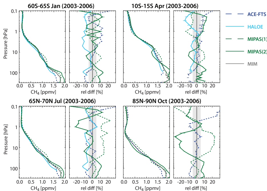
Figure 4.3.2: Vertical profiles of monthly zonal mean \text{CH}_4 for 2003-2006. Vertical \text{CH}_4 profiles for 60°S-65°S January and 10°S-15°S April (upper panels) and for 65°N-70°N July and 85°N-90°N October (lower panels) are shown together with their differences from the MIM. HALOE, MIPAS(1), ACE-FTS, and MIPAS(2) data are averaged over the years 2003-2005, 2003-2004, 2004-2006, and 2005-2006, respectively, according to their availability within this time period.
