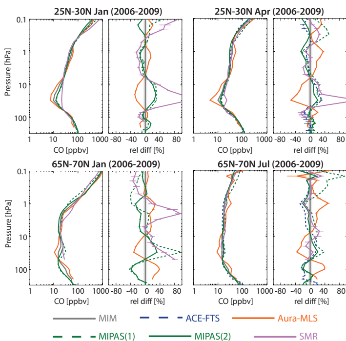
Figure 4.7.2b: Vertical profiles of monthly zonal mean CO for 2006-2009. Vertical CO profiles for January and April 25°N–30°N (upper panels), and for January and July 65°N–70°N (lower panels) are shown together with instrument differences from the MIM. Note, SMR and MIPAS(1) measurements are taken in 2003–2004 and 2002–2004, respectively.
