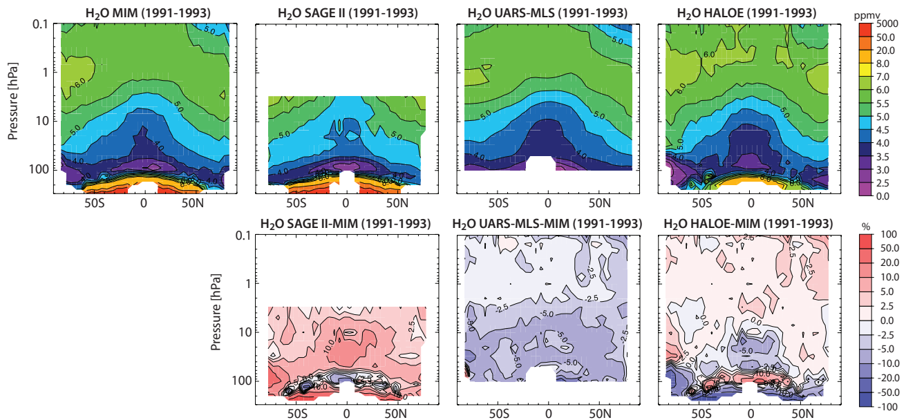
Figure 4.2.2: Cross sections of annual zonal mean \text{H}_2\text{O} and differences for 1991-1993. Shown from left to right are the MIM, SAGE II, UARS-MLS, and HALOE. Upper panels show absolute values, lower panels the differences relative to the MIM.
