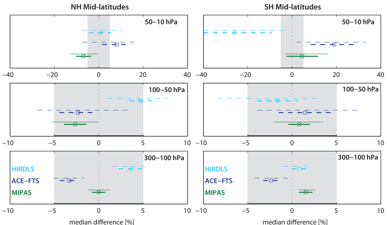
Figure 4.6.8b: Summary CFC-12 differences in mid-latitudes for 2005-2007. Like Figure 4.6.8a but for NH mid-latitudes ( 30^{\circ}\text{N} - 60^{\circ}\text{N} ) and SH mid-latitudes ( 30^{\circ}\text{S} - 60^{\circ}\text{S} ).
