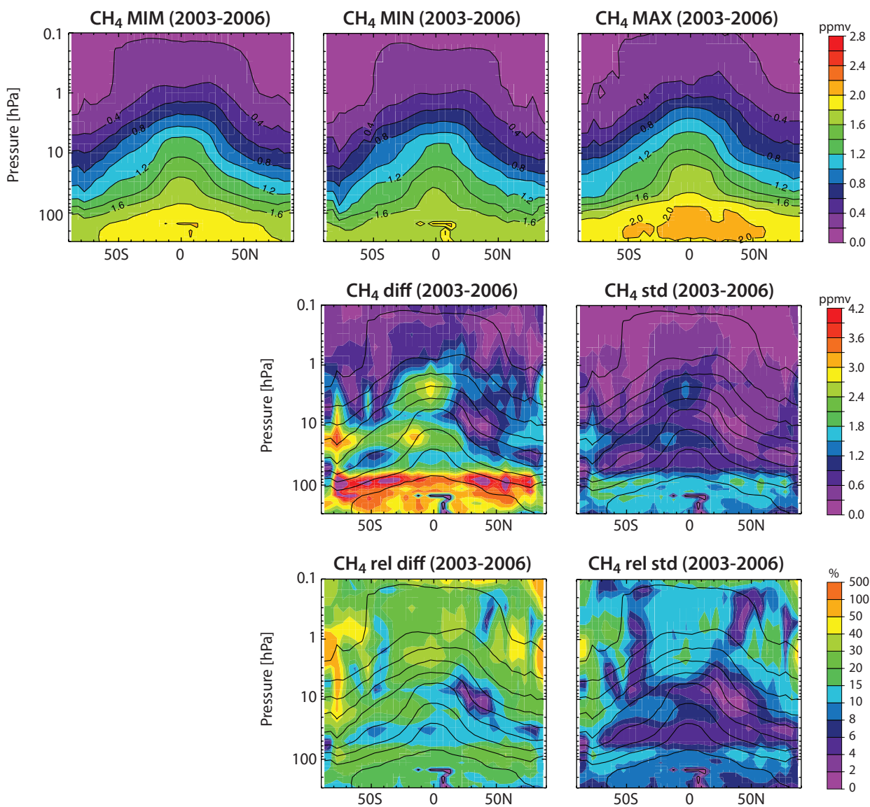
Figure 4.3.6: Summary of CH 4 annual zonal mean state for 2003-2006. Annual zonal mean cross sections for 2003-2006 of the MIM, minimum (MIN), and maximum (MAX) CH 4 values are shown in the upper row. The maximum differences over all instruments (MAX-MIN) and the standard deviation over all instruments are shown in the middle row. The relative differences and relative standard deviations with respect to the MIM are shown in the lower row. Black contours in lower panels repeat the MIM distribution. Instruments considered are HALOE, MIPAS(1), ACE-FTS, and MIPAS(2).
