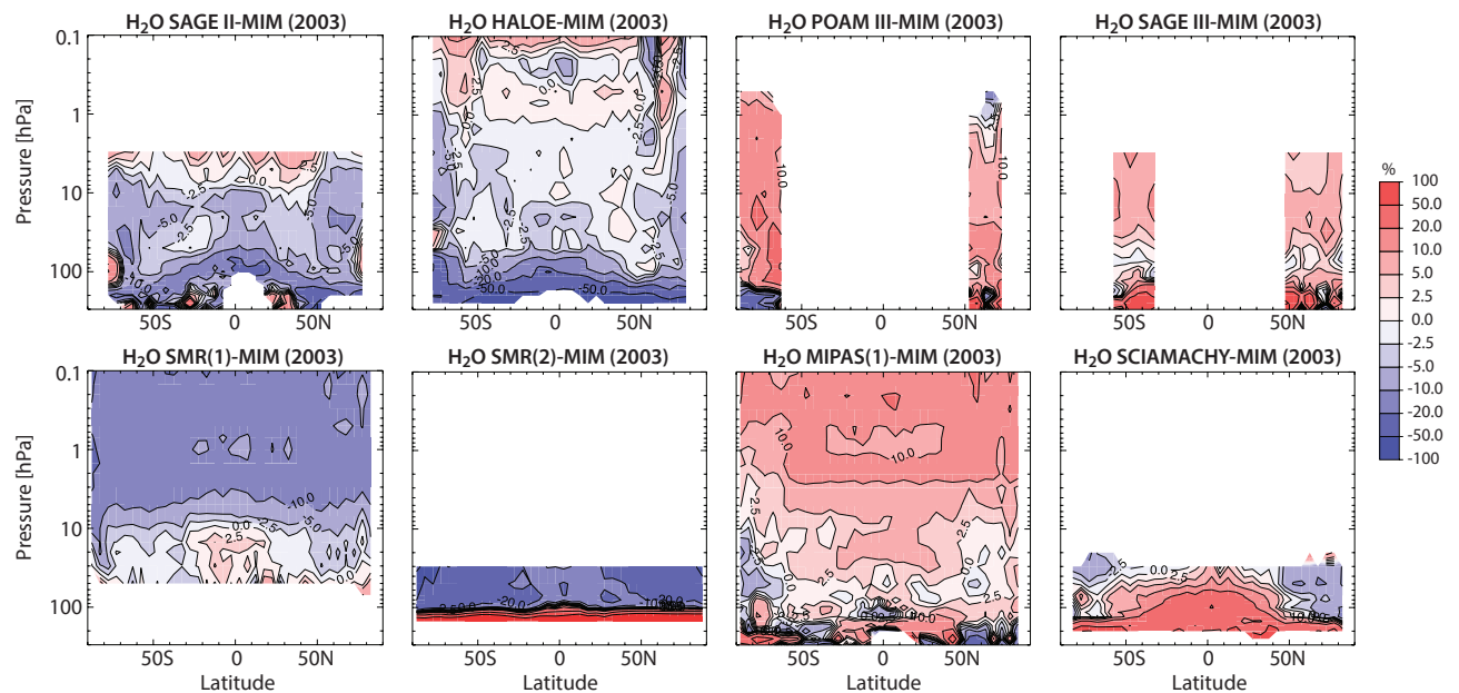
Figure 4.2.8b: Cross sections of annual zonal mean \text{H}_2\text{O} differences for 2003. Relative differences with respect to the MIM are shown for the individual instruments shown in Figure 4.2.8a. Note that SMR(2) is not included in the MIM.
