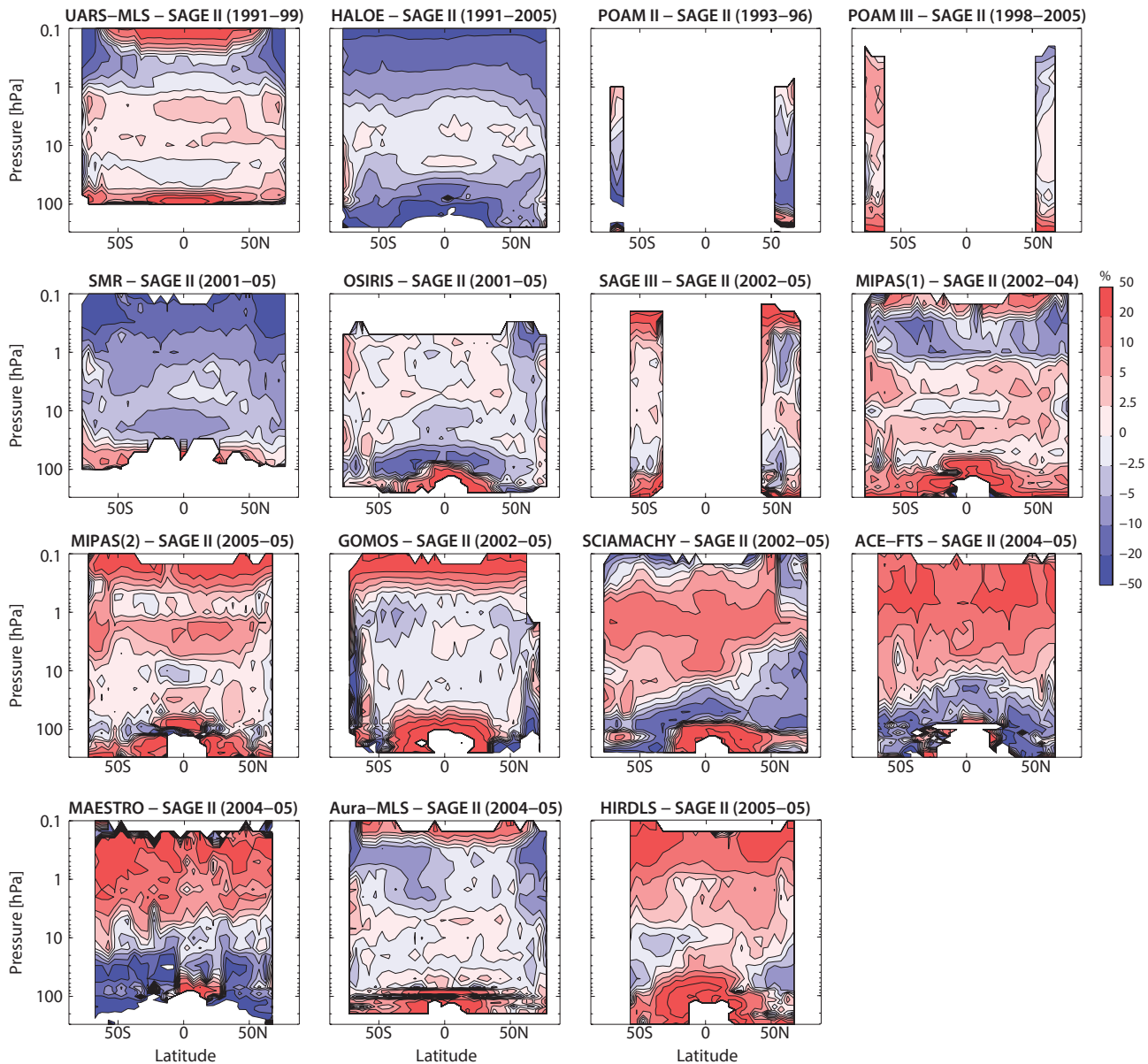
Figure 4.1.18: Cross sections of zonal mean ozone differences to SAGE II. Zonal mean ozone differences between the individual instruments and SAGE II are shown for time periods of maximum overlap.
