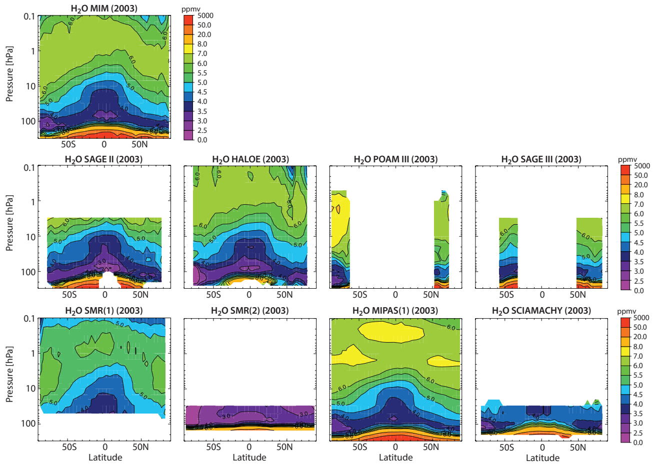
Figure 4.2.8a: Cross sections of annual zonal mean \text{H}_2\text{O} for 2003. Shown are the annual mean cross sections for the MIM (upper row), SAGE II, HALOE, POAM III, SAGE III (middle row), and SMR(1), SMR(2), MIPAS(1), and SCIAMACHY (lower row). Note that SMR(2) is not included in the MIM.
