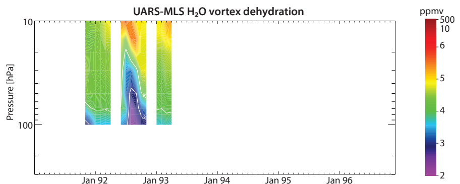
Figure 4.2.20: Polar vortex dehydration. Southern Hemisphere polar vortex descent and dehydration as observed in UARS-MLS in the Antarctic polar vortex 60^\circ\text{S} – 90^\circ\text{S} between 1991 and 1993.
