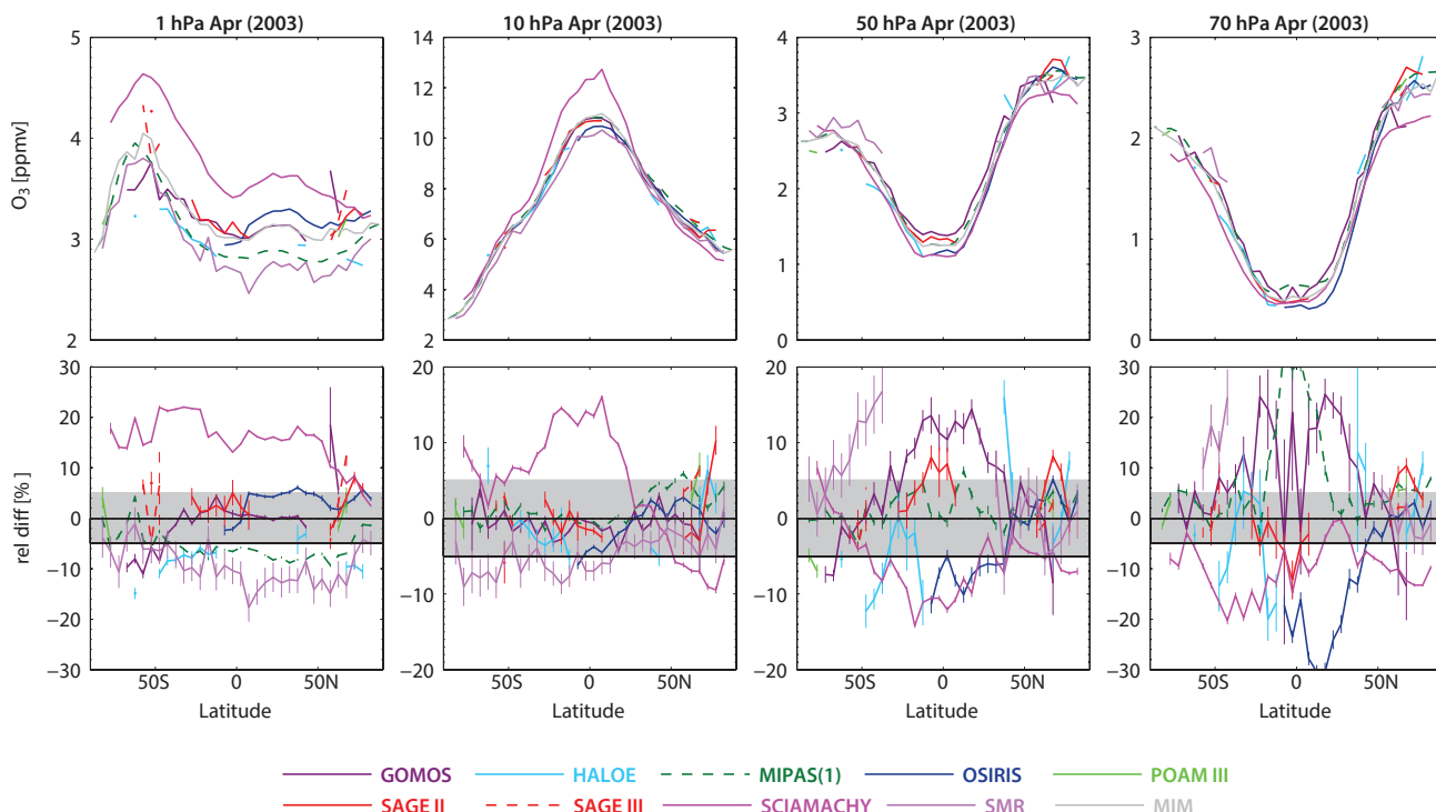
Figure 4.1.9: Meridional profiles of monthly zonal mean ozone for 2003. Meridional zonal mean ozone profiles at 1, 10, 50 and 70 hPa for April 2003 are shown in the upper row. Differences between the individual instruments and the MIM profiles are shown in the lower row. Error bars indicate the uncertainties in each climatological mean based on the SEM. The grey shaded area indicates where relative differences are smaller than \pm 5\% .
