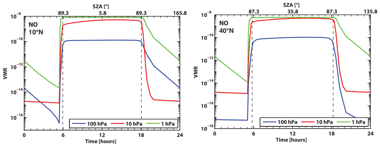
Figure 4.10.1: Diurnal NO cycle. NO variations as function of LST are shown at 10^\circ N and 40^\circ N at 1, 10, and 100 hPa for March 15.
