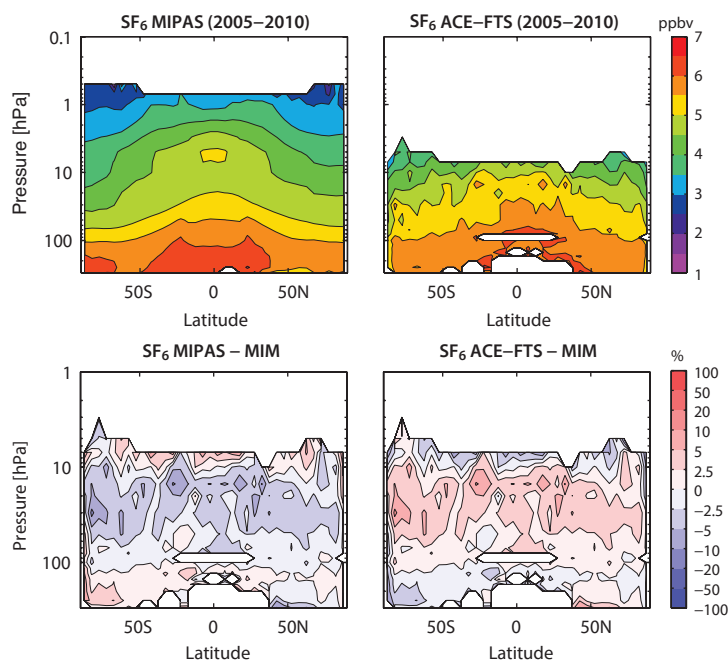
Figure 4.9.1: Cross sections of annual zonal mean SF_6 for 2005–2010. SF_6 cross sections are shown for MIPAS and ACE-FTS.
