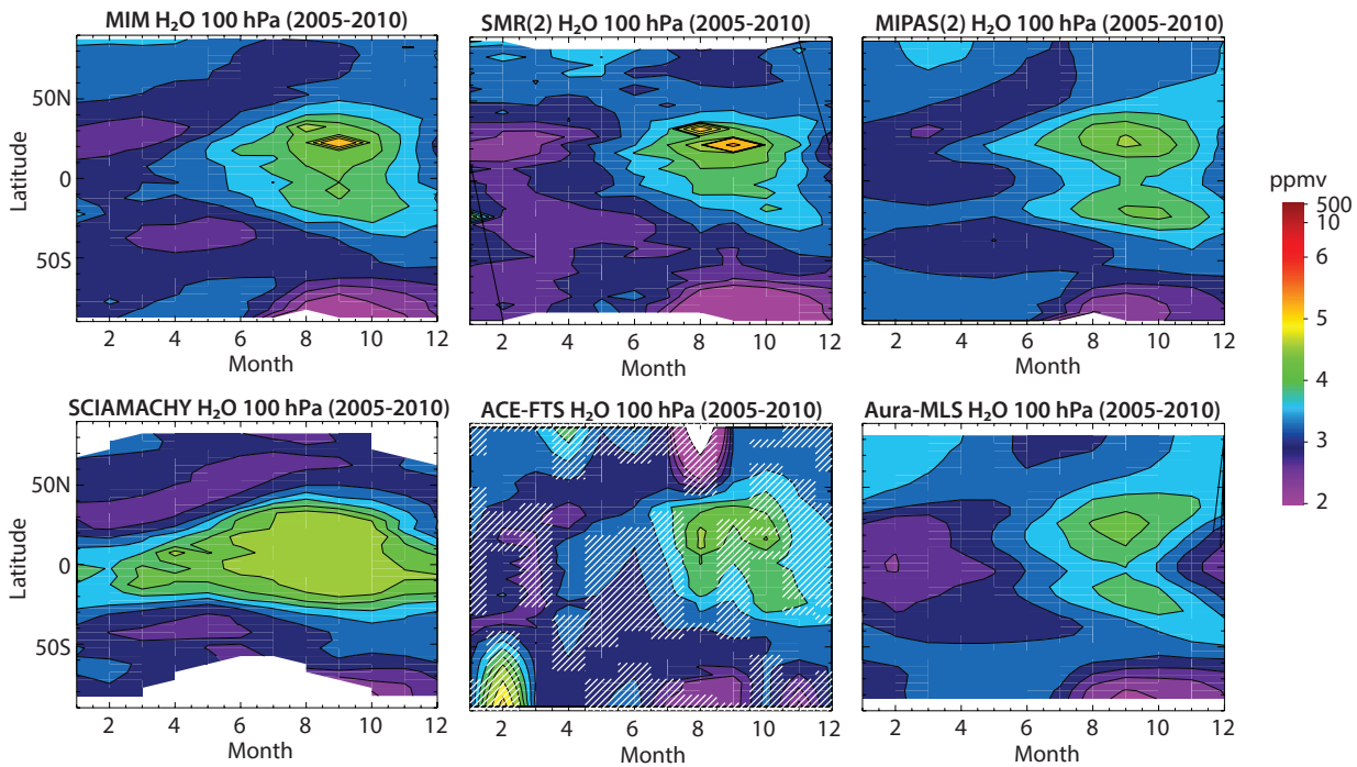
Figure 4.2.19: The horizontal tape recorder during 2005–2010. Shown is a latitude-time evolution of \text{H}_2\text{O} at 100 hPa averaged over this period. ACE-FTS shows interpolated data; white hatching indicates the areas where no data was available. Note the differences in Aura-MLS, SMR(2), and SCIAMACHY when compared to the earlier time period (Figure 4.2.18).
