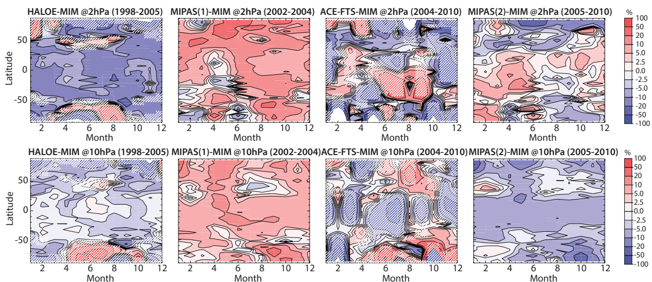
Figure 4.3.4b: Latitude–time evolution of differences in \text{CH}_4 . \text{CH}_4 differences with respect to the MIM at 2 hPa (top), and 10 hPa (bottom) are shown for HALOE, MIPAS(1), ACE-FTS, and MIPAS(2) over the time period as indicated in Figure 4.3.4a. For HALOE and ACE-FTS, hatched regions indicate where no measurements are available.
