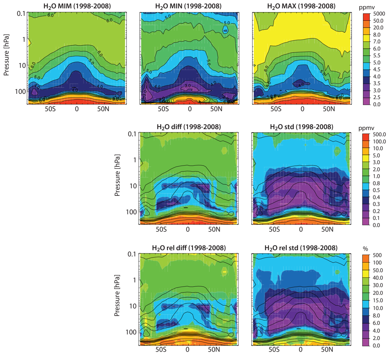
Figure 4.2.23: Summary of \text{H}_2\text{O} annual zonal mean state for 1998-2008. Shown are the annual zonal mean cross sections of the MIM, minimum (MIN) and maximum (MAX) \text{H}_2\text{O} values (upper row), the absolute differences (MAX-MIN) and absolute standard deviations (middle row), and relative differences and relative standard deviations with respect to the MIM (lower row). Black contour lines in the lower panels repeat the MIM distribution. Instruments considered are SAGE II, SAGE III, HALOE, POAM III, ACE-FTS, Aura-MLS, MIPAS, SAGE III, SMR(1), and SCIAMACHY.
