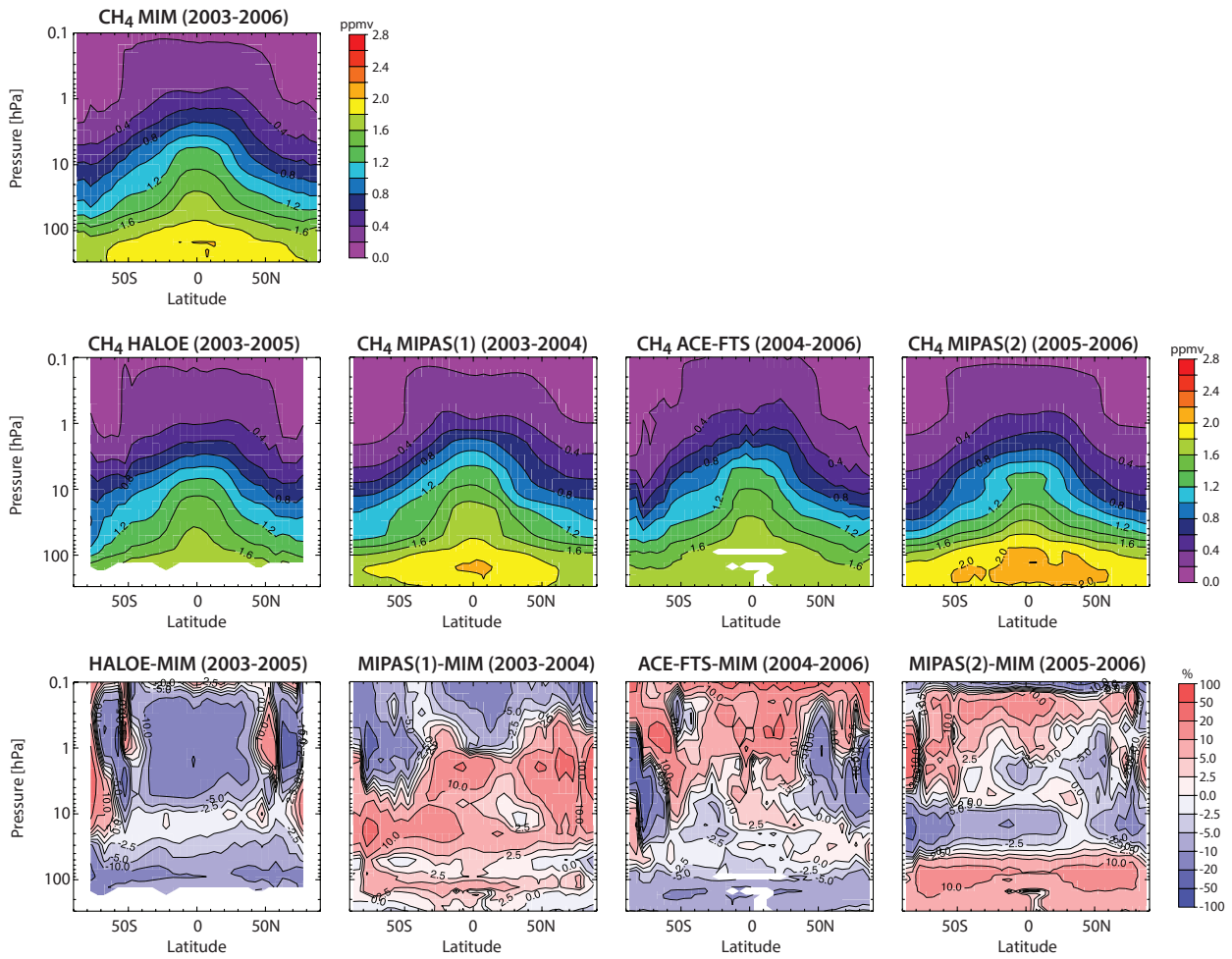
Figure 4.3.1: Cross sections of annual zonal mean \text{CH}_4 for 2003-2006. Upper panel shows the \text{CH}_4 cross section for the MIM, middle panels show cross sections for the different instruments (HALOE, MIPAS(1), ACE-FTS, and MIPAS(2)), and lower panels show the relative differences between each instrument and the MIM.
