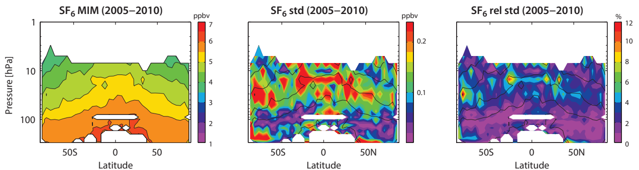
Figure 4.9.7: Summary of \text{SF}_6 annual zonal mean state for 2005–2010. Shown are the annual zonal mean cross section of the \text{SF}_6 MIM (left panel), the standard deviation over both instruments (middle panel), and the relative standard deviation with respect to the MIM (right panel). Black contour lines in the right panels give the MIM distribution. Instruments included are MIPAS and ACE-FTS. The MIM and standard deviation are only displayed for regions where both instruments provide measurements.
