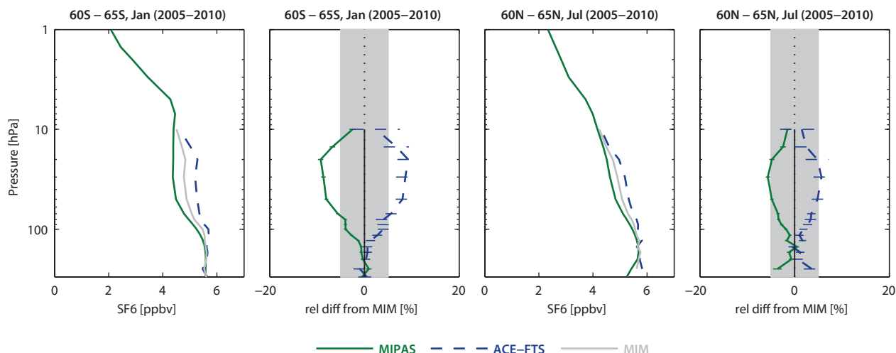
Figure 4.9.3: Vertical profiles of monthly zonal mean \text{SF}_6 for 2005-2010. Zonal mean \text{SF}_6 profiles for 60°S-65°S, January (left panels) and 60°N-65°N, July (right panels) are shown together with their differences from the MIM. The grey shading indicates the \pm 5\% difference range. Bars indicate the uncertainties in the relative differences.
