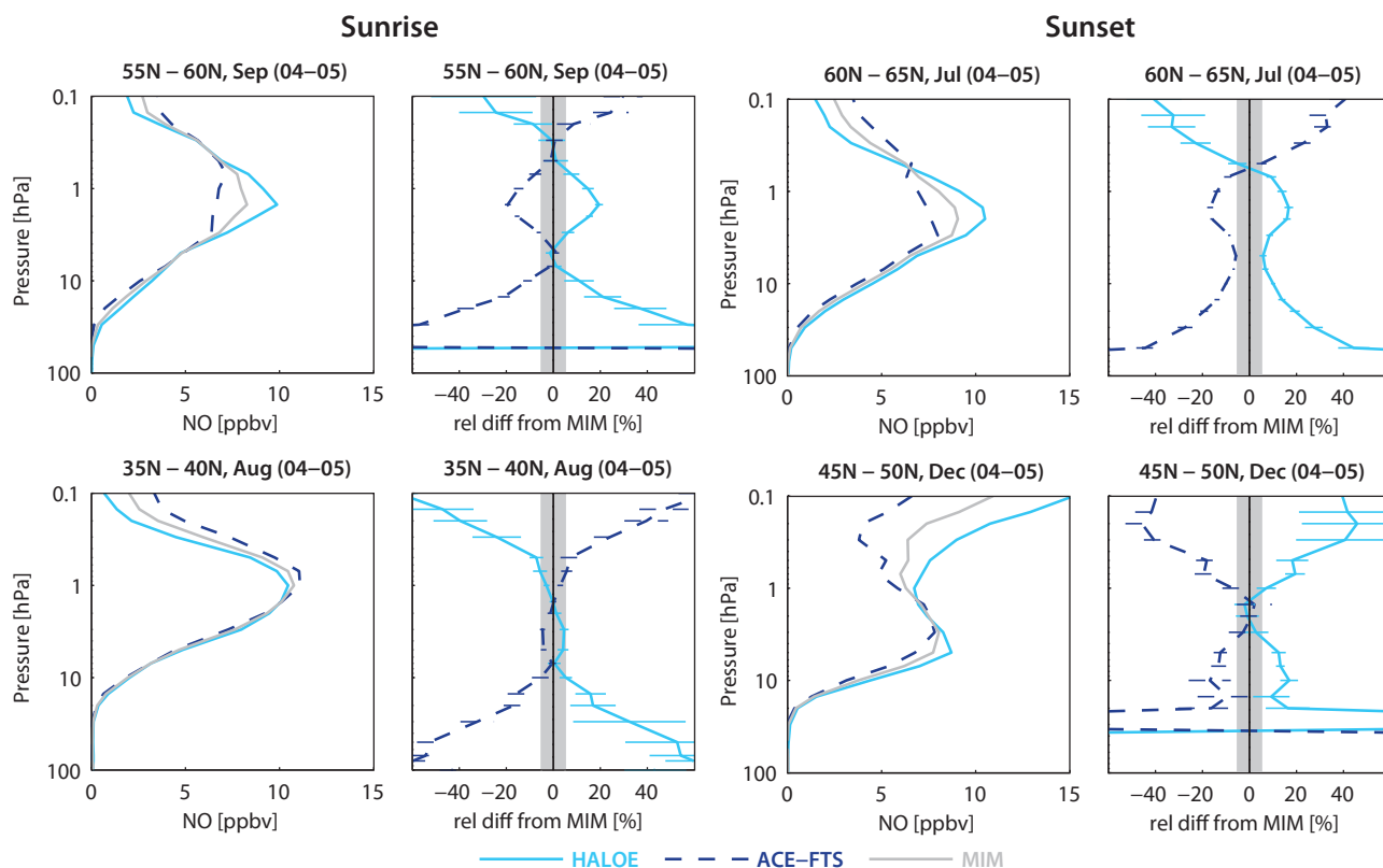
Figure 4.10.4: Profiles of monthly zonal mean, local sunrise and sunset NO for 2004-2005. Zonal mean NO profiles are shown together with their differences from the MIM for local sunrise, 55°N-60°N, September and 35°N-40°N, August (column 1 and 2) and local sunset, 60°N-65°N, July and 45°N-50°N, December (column 3 and 4).
