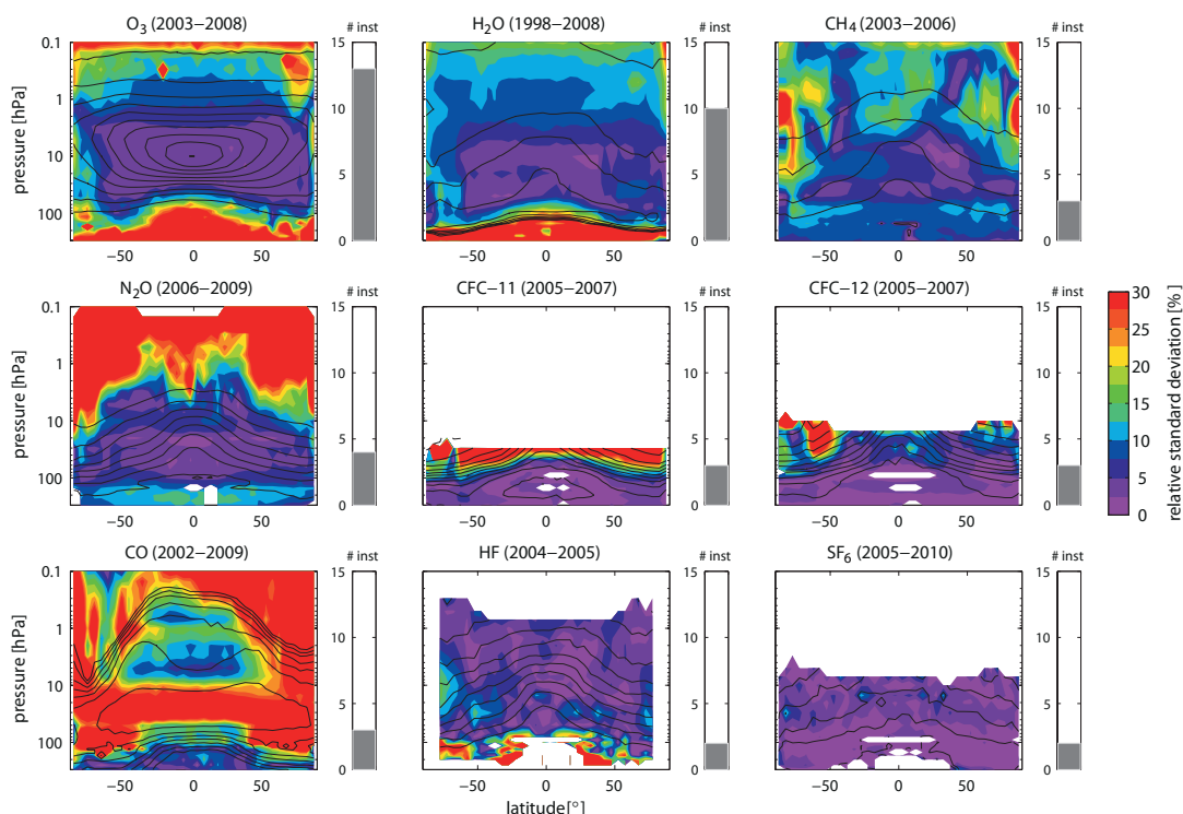
Figure ES.1: Synopsis of the uncertainty in the annual zonal mean state of longer-lived species. The relative standard deviation over all instruments' multi-annual zonal mean datasets is presented for O_3 , H_2O , CH_4 , N_2O , CFC-11, CFC-12, CO, HF, and SF_6 (colour contours). The relative standard deviations are calculated by dividing the absolute standard deviations by the multi-instrument mean (MIM). The black contour lines in each panel represent the MIM trace gas distribution for each species. The number of instruments included is given by the right-hand grey bar, while detailed information on which instruments are included can be found in the respective trace gas sections. Note that the time periods used depend on the availability of the instruments included in the assessment and hence differ from trace gas to trace gas.
