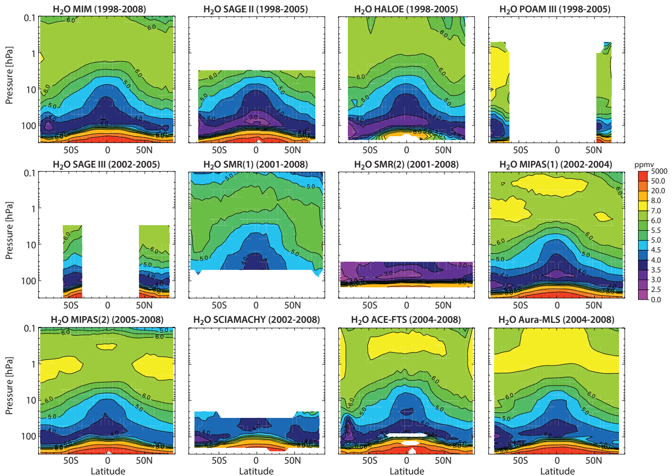
Figure 4.2.11a: Cross sections of annual zonal mean \text{H}_2\text{O} for 1998-2008. Shown are the MIM, SAGE II, HALOE, POAM III (upper row), SAGE III, SMR(1), SMR(2), MIPAS(1) (middle row), and MIPAS(2), SCIAMACHY, ACE-FTS, and Aura-MLS (lower row). Note, SMR(2) and MIPAS(1) are not included in the MIM.
