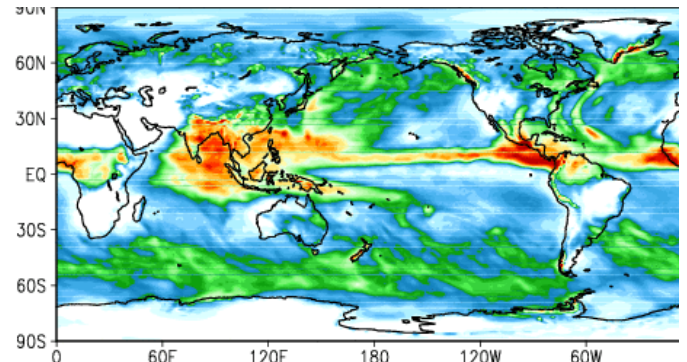
RHcrit from Original AGCM
