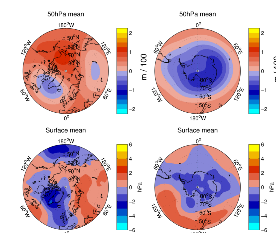
Figure 9: Ensemble mean, post-volcanic anomalies from the ECHAM6 runs in first NH winter (DJF-1, a and c) and first SH spring (SON-1, b and d).
