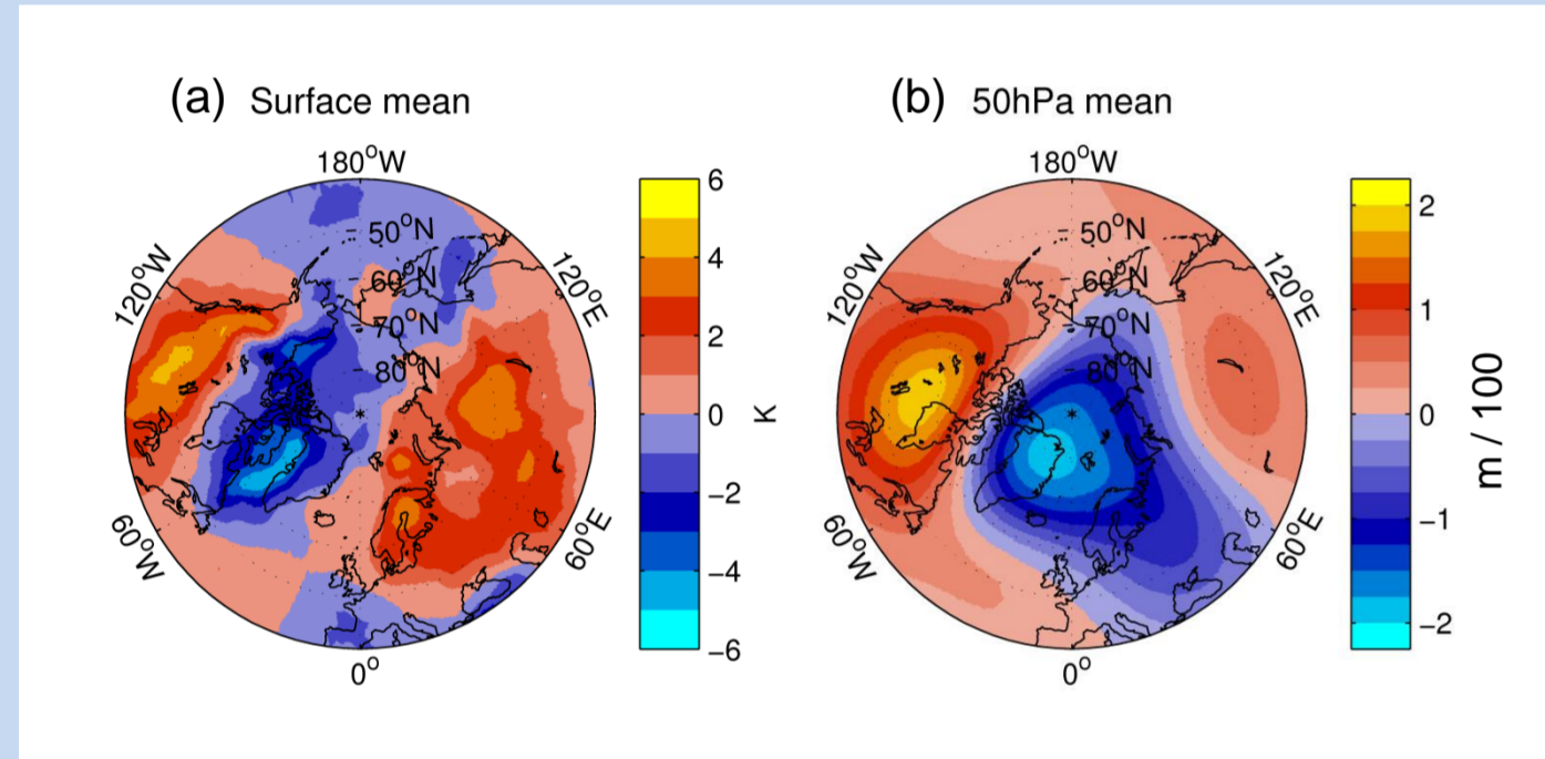
Figure 1: ERA-40 NH winter (DJF) surface temperature (a) and 50 hPa geopotential height (b) anomalies from the seasonal 9-year running mean, averaged over years 1991/92 and 1982/83, the first winters after the Pinatubo and El Chichón eruptions.
