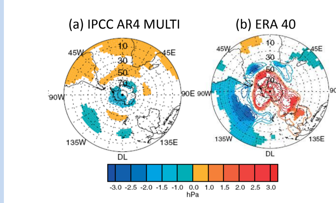
Figure 2: SH spring (OND) mean detrended SLP anomalies averaged over years 1982 and 1992 for IPCC AR4 multi-model ensemble mean (MULTI) and ERA-40, from Karpechko et al. (2010).
