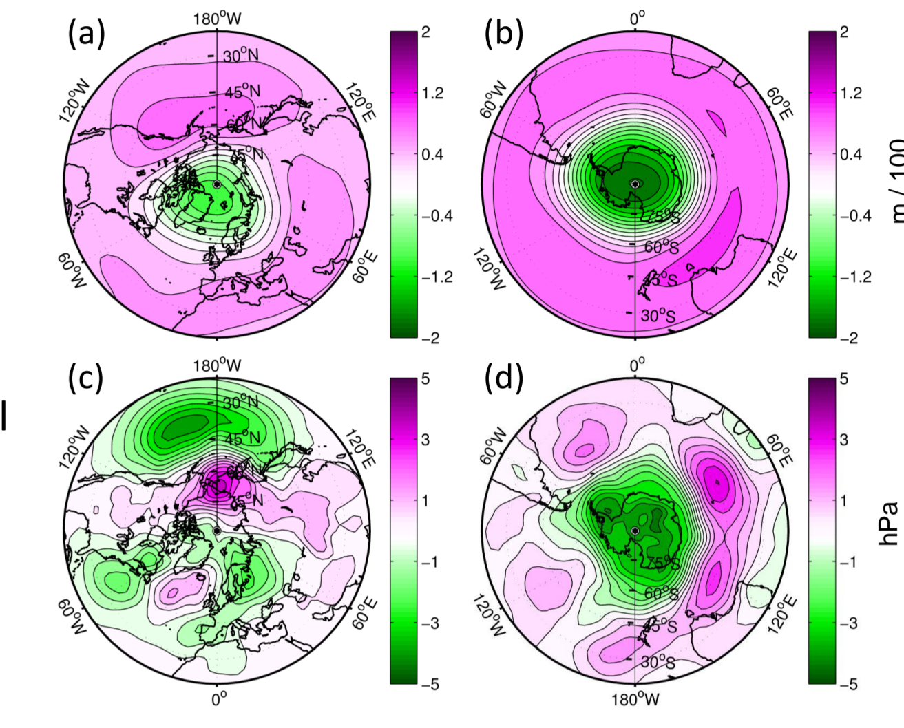
Figure 5: Ensemble mean geopotential height and SLP anomalies from the MAECHAM5-HAM runs in first NH winter (DJF-1, a and c) and first SH spring (OND-1, b and d).
