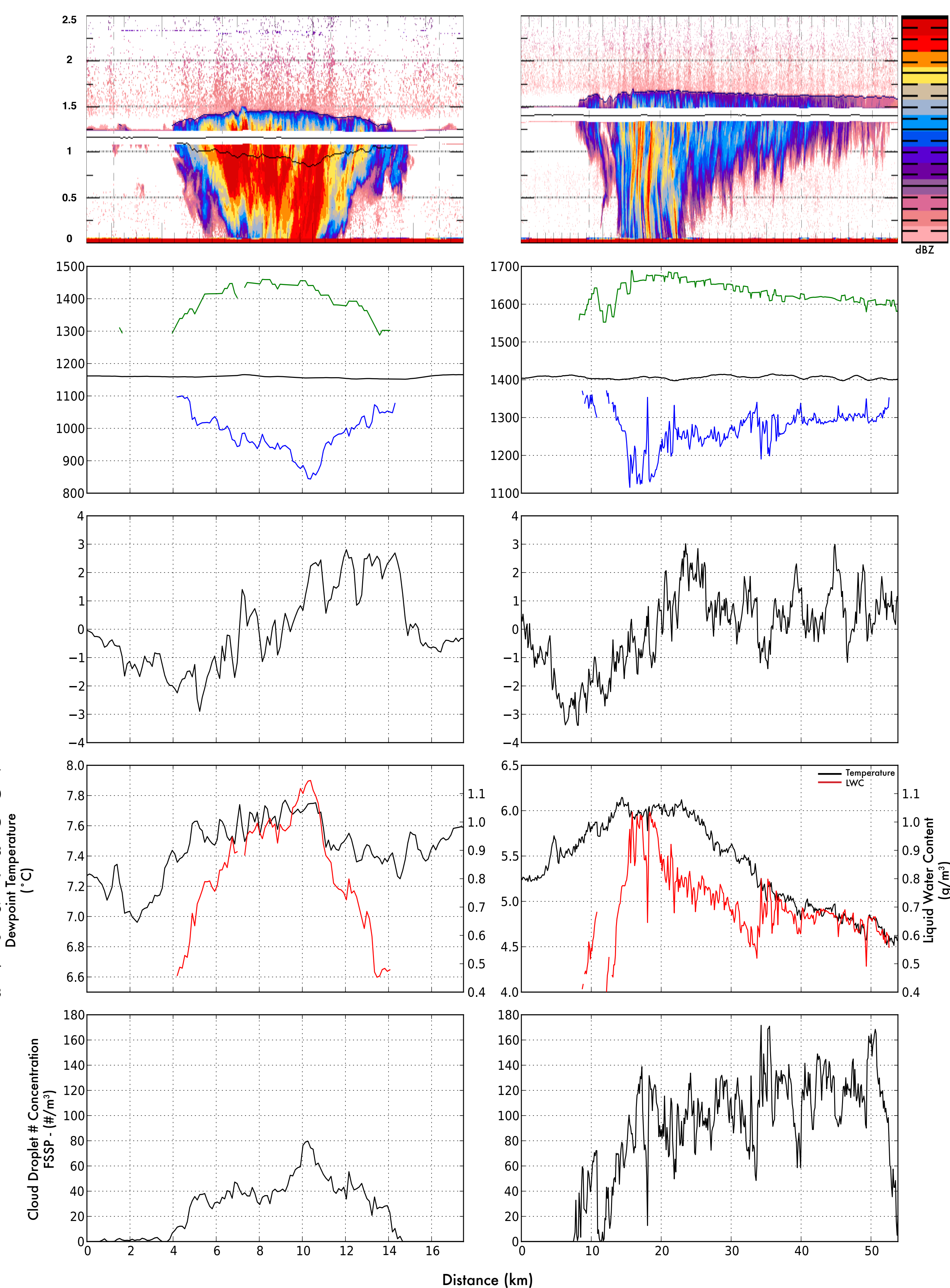
Cell selection from research flight 6. This flight was a 'POC' flight, which sampled pockets of open cellular convection. This cell was located at 18.14°S, 79.95°W.
