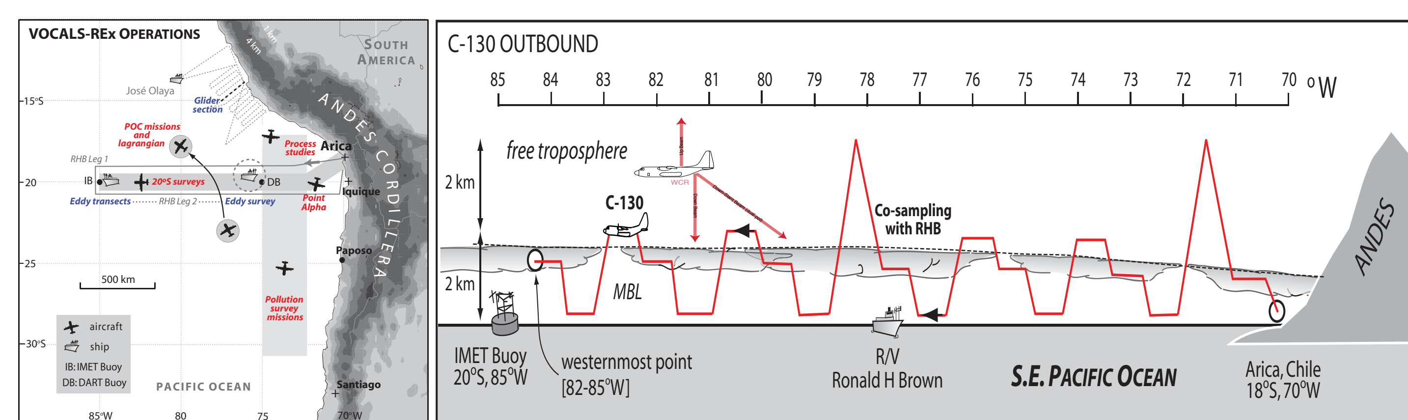
Schematic of the VOCALS REx study region (top left) outlining the observational strategy. 20°S survey flights are detailed in the right figure (Wood 2011) with C-130 detailed diagram of the Wyoming Cloud Radar placement.
