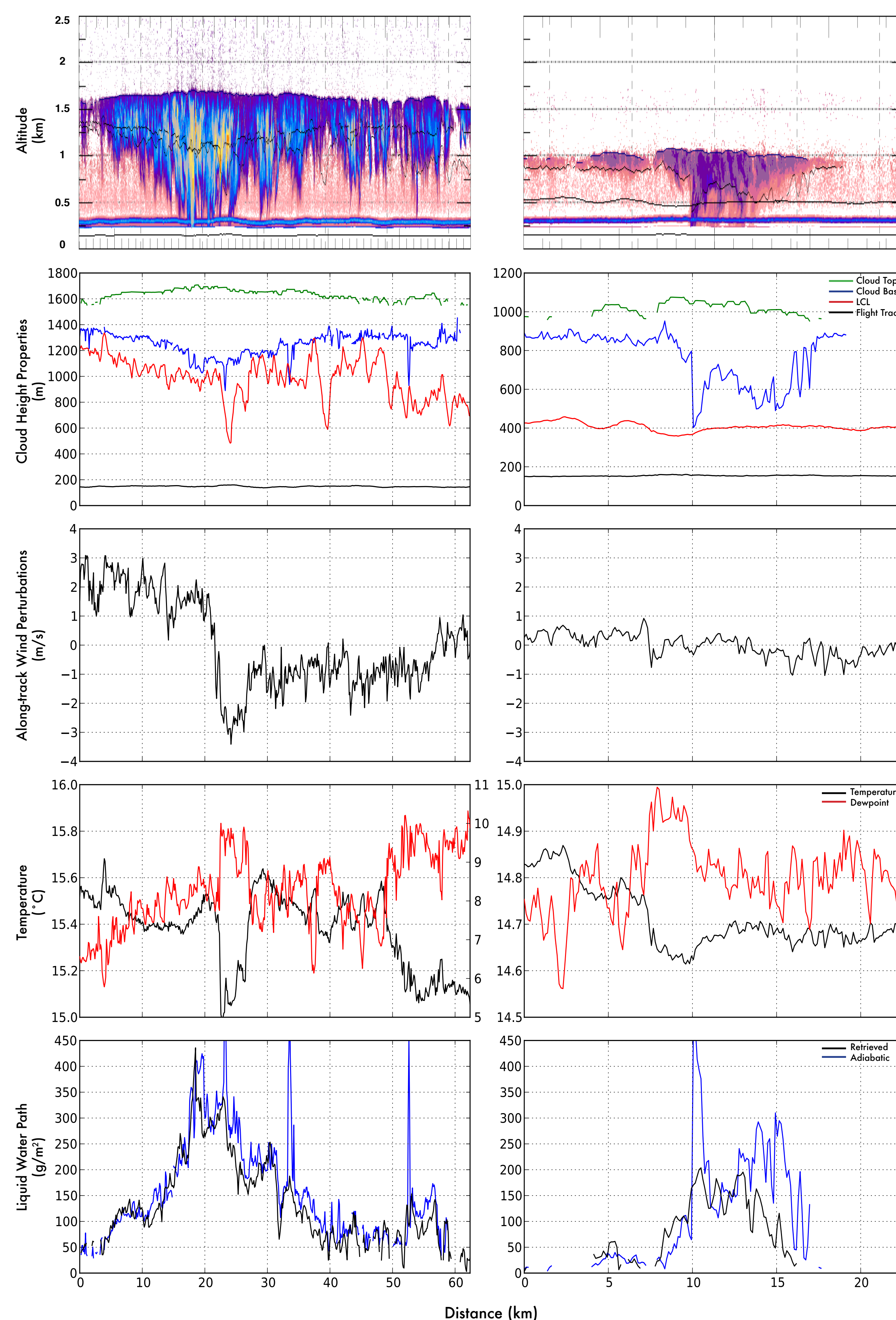
Cell selection from research flight 7. This cell was located at 23.34°S, 80.09°W and was sampled from a deep layer of stratocumulus clouds.
