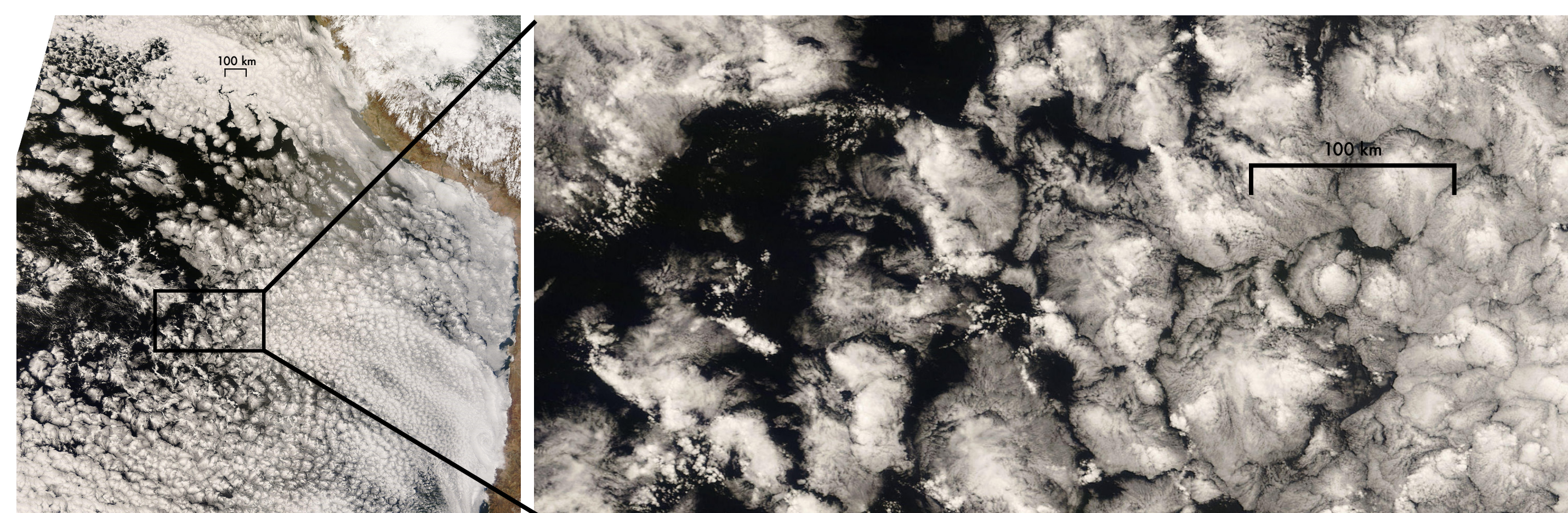
MODIS image showing the typical structure of the SEP stratocumulus deck. Spatial variability of mesoscale organization in this region varies from several kilometers to hundreds of kilometers.
